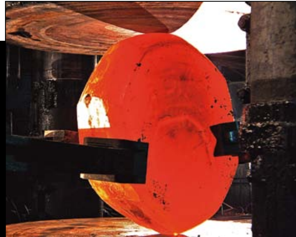
▲ At a forging plant in Wisconsin, the titanium ingots were heated to 1,700°F and "edge rolled" to get them as close to circular as possible. Next, they were paddled to flatten them and to reduce their thickness to about 6 inches.
